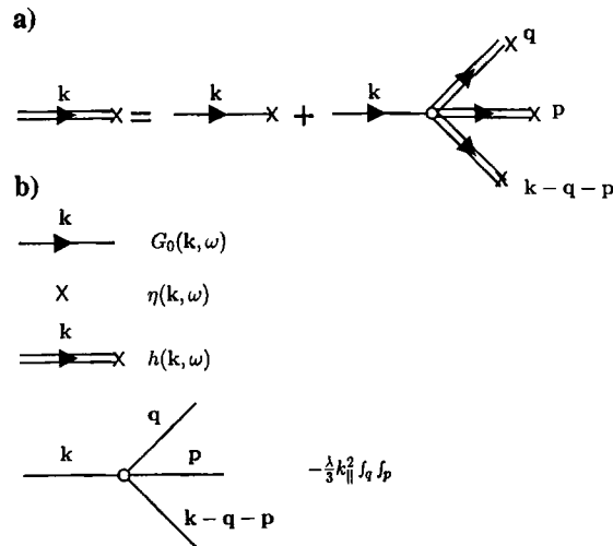
Fig. 7. (a) Diagrammatic expansion of Eq. (A3) of Feynman diagrams. (b) Definition of the various terms.
