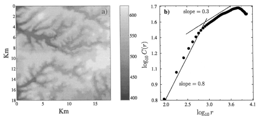
Fig. 2. (a) Digital elevation map of an area of the Appalachian Plateau, in Northwest Pennsylvania. Elevations are given in meters. The spatial resolution is 90 m. (b) Averaged height-height correlation function C(r) for the landscape in Fig. 2a, where r is oriented in the vertical direction of (a). A plot of similar shape, but with smaller values of C(r) , is obtained in the horizontal case. Logarithms are computed from quantities measured in units of meters.
