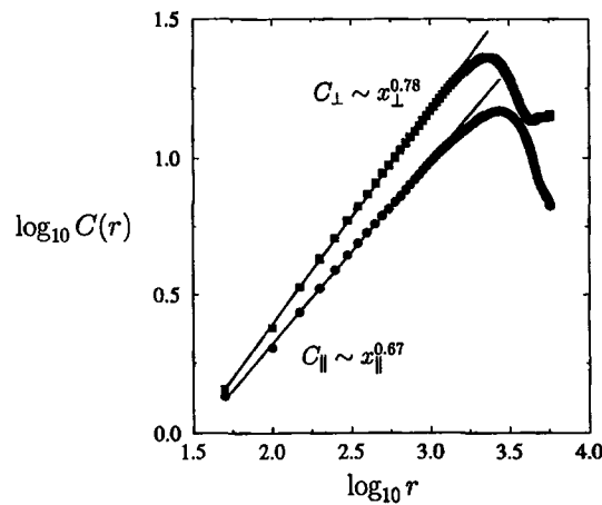
Fig. 4. Height-height correlation functions computed along the parallel ( C_{\parallel} ) and perpendicular ( C_{\perp} ) directions for the landscape shown in Fig. 3a. Solid lines are least-squares fits to the scaling region. The logarithms are computed from quantities measured in meters.
