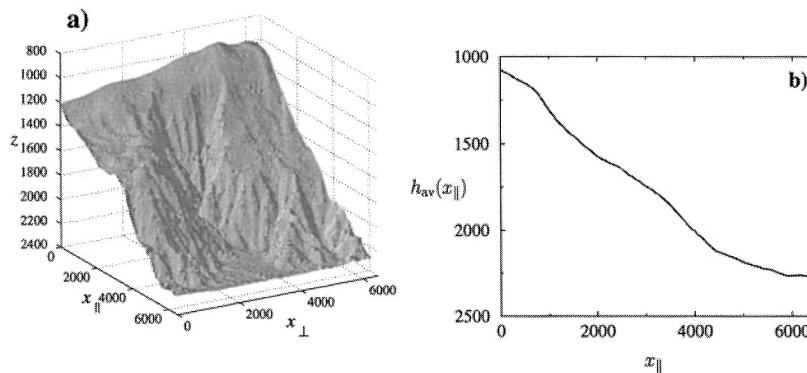
Fig. 3. (a) Digital map of a submarine canyon off the coast of Oregon, located at coordinates 44^{\circ}40'N , 125^{\circ}45'W . The vertical axis represents the depth z below sea level. The spatial resolution is 50 m. (b) Mean average profile of the canyon, along the direction x_{\parallel} . All units are given in meters.
