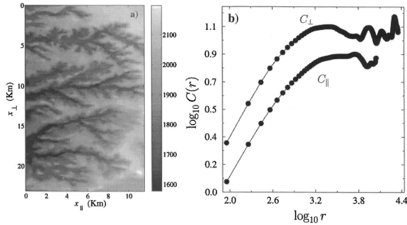
Fig. 5. Digital elevation map of an area near Marble Canyon, in Northeast Arizona. Elevations are given in meters, and the spatial resolution is 90 m. (b) Height-height correlation functions computed along the parallel ( C_{\parallel} ) and perpendicular ( C_{\perp} ) directions for the landscape shown in Fig. 5a. Logarithms are computed from quantities measured in meters.
